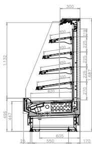
Fjorda 2020 SSL 4.5 R
