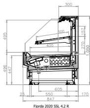
Fjorda 2020 SSL 4.2 R
