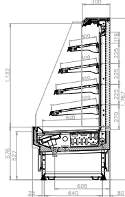
Fjorda 2020 SSL 5.5 R
