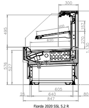
Fjorda 2020 SSL 5.2 R
