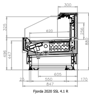
Fjorda 2020 SSL 4.1 R
