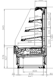
Fjorda 2020 SSL 5.4 R
