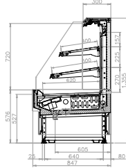
Fjorda 2020 SSL 5.3 R
